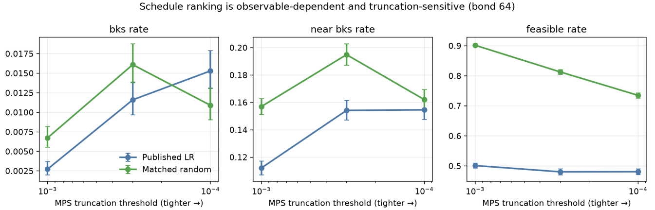
Figure 2: Observable-dependent convergence at fixed bond dimension 64. Tightening the threshold reverses the BKS ranking between 3 \times 10^{-4} and 10^{-4} , while near-BKS and feasible rankings remain unchanged. The 10^{-3} point uses 15,000 shots; the other points use 10,000 shots per method.
