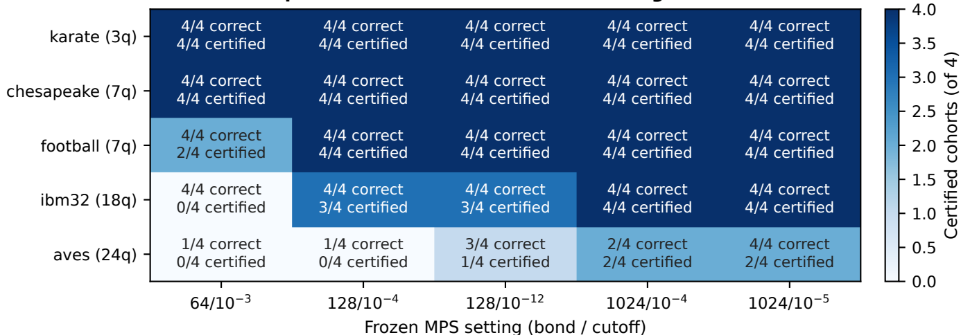
c Per-case replication across backend and ordering
