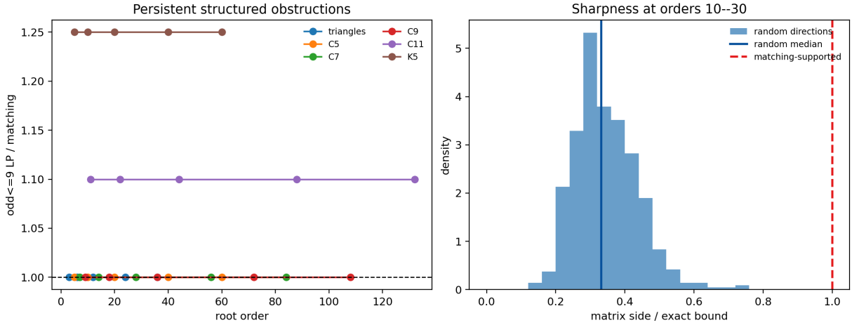
Figure 4: Left: local obstructions persist under direct sums. Right: generic Gaussian directions are far from equality while matching-supported directions remain exactly sharp.
