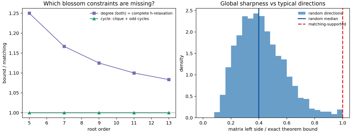
Figure 2: Mechanism ablations. Odd cycles repair cycle roots but not odd complete roots; removing skewness violates the blossom constraint; random directions are usually nonsaturating although equality is globally attainable.
