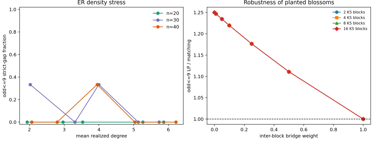
Figure 5: Density and weak-coupling stress. Random exactness is nonmonotone, whereas planted blossom gaps survive connectivity and weak bridges with a size-independent curve.
