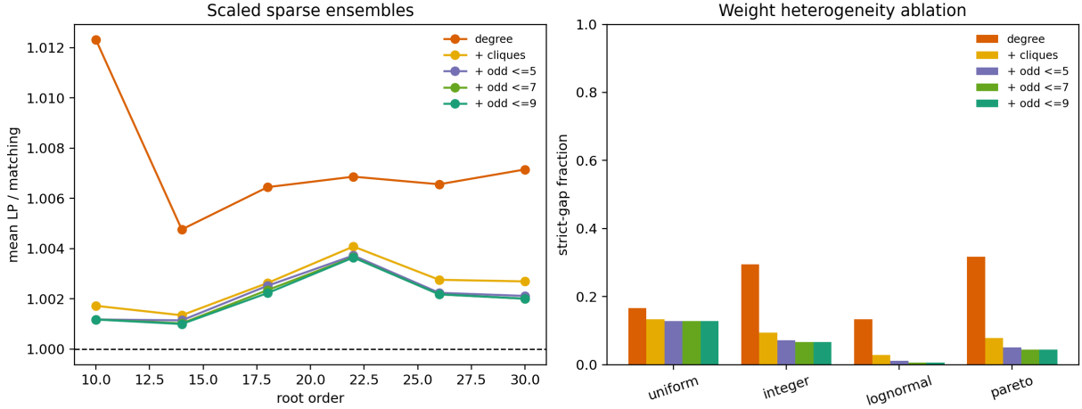
Figure 3: Scaling and weight ablations on 720 weighted sparse instances. Local constraints usually make the remaining gap small, but exactness depends on the graph and weight ensemble.
