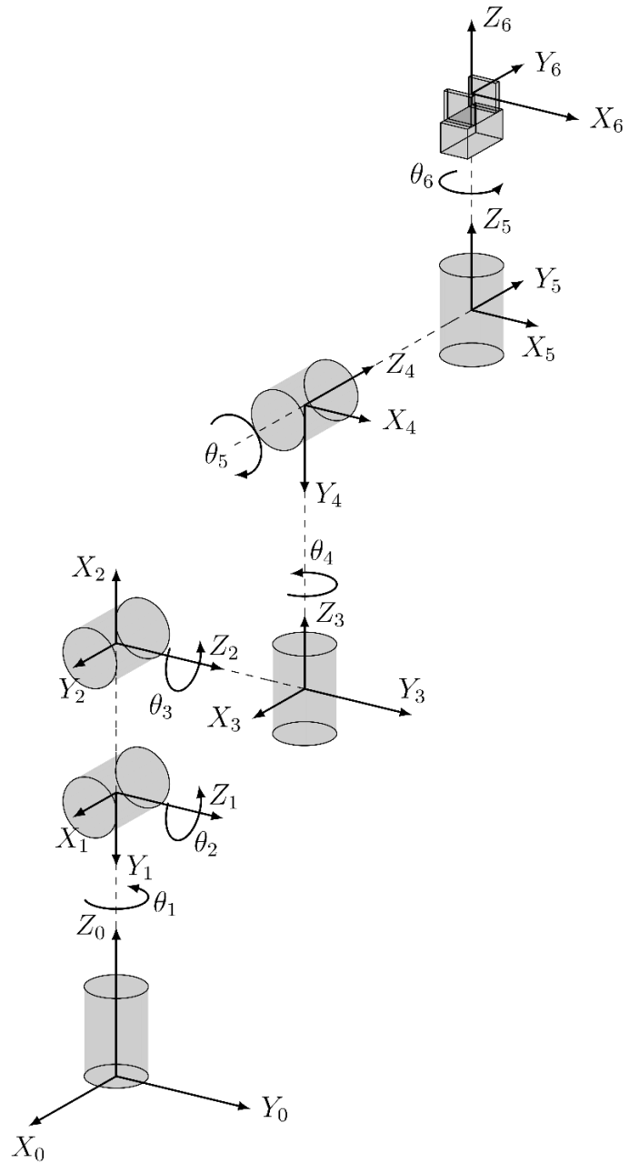
Figure: Kinematic diagram of the robotic arm.
