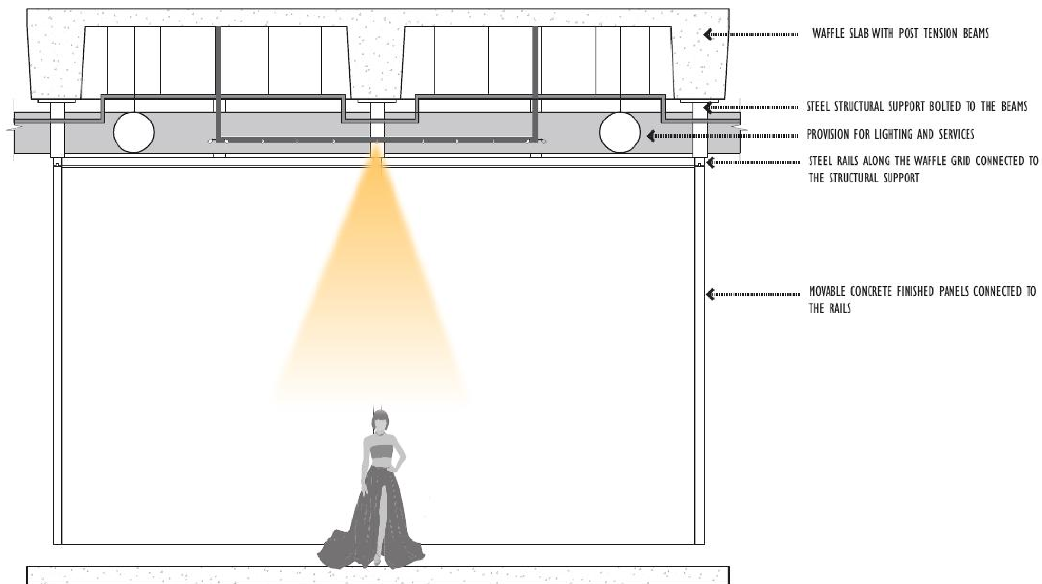
MOVABLE PANEL CONNECTION SCALE 1:25
