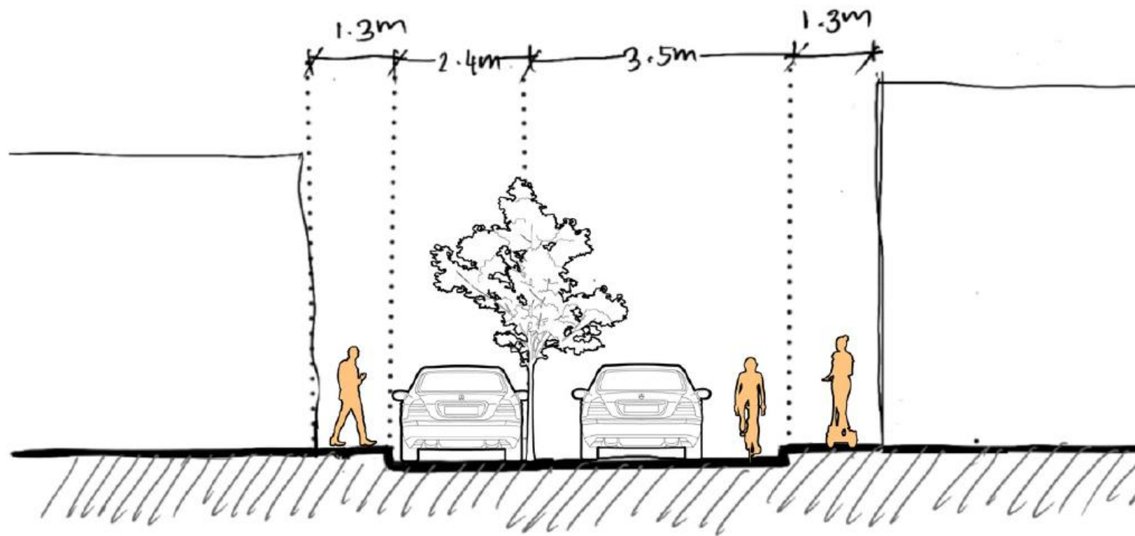
STREET SECTION OF CULBITT ST WITH PARKING
