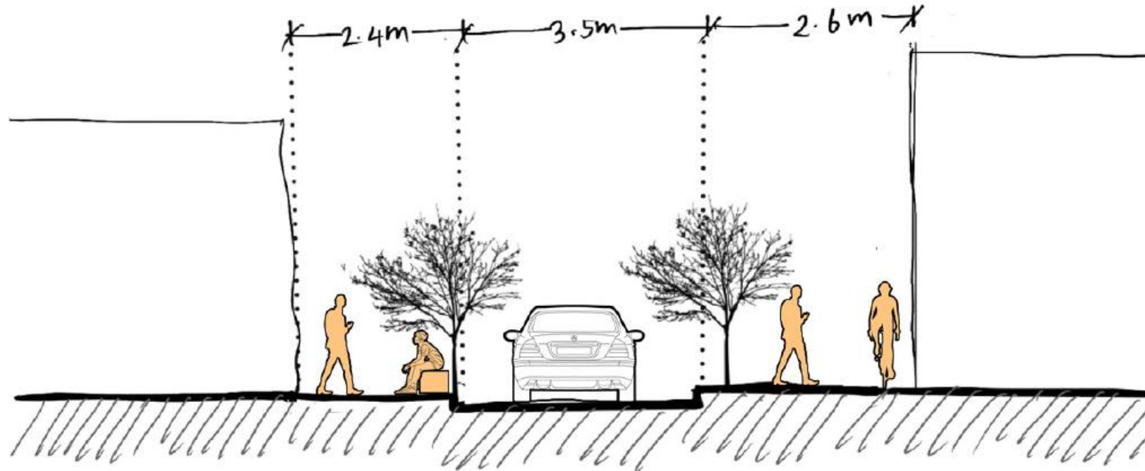
STREET SECTION OF CULBITT ST WITHOUT PARKING
