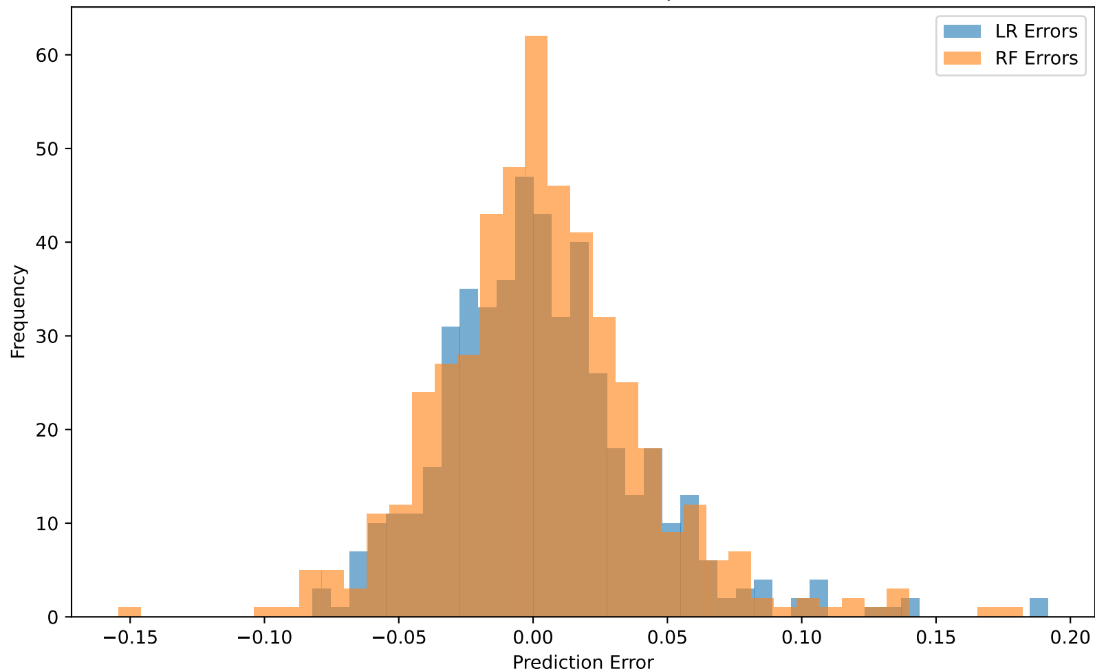
Error Distribution Comparison
