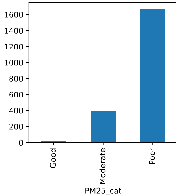
PM2.5
