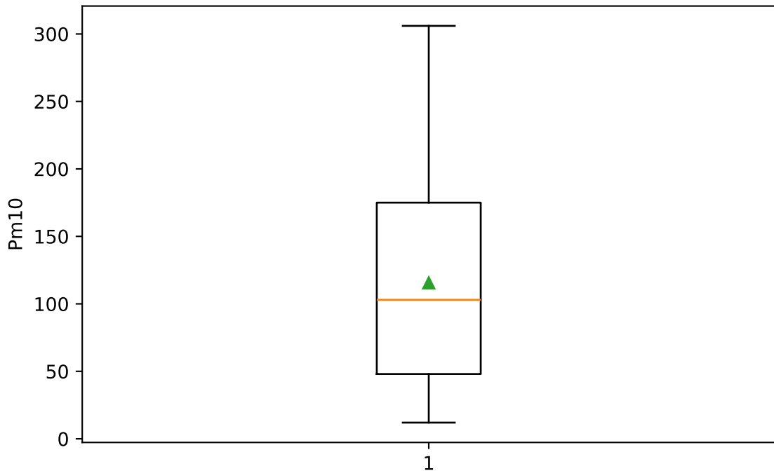
Outlier Detection (IQR) — Pm10
