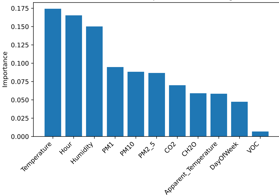
Random Forest Feature Importances for O3 Regression
