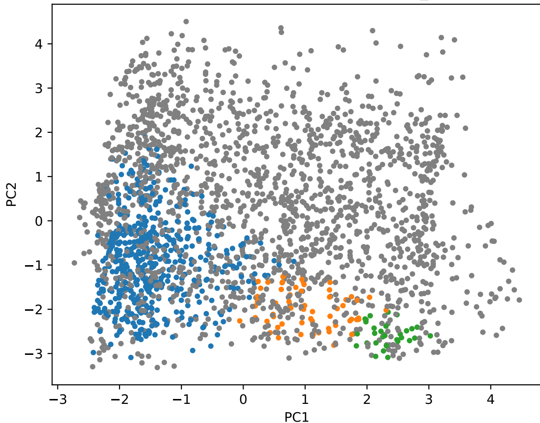
DBSCAN Clusters in PCA Space (eps=1.0, min_samples=30)
