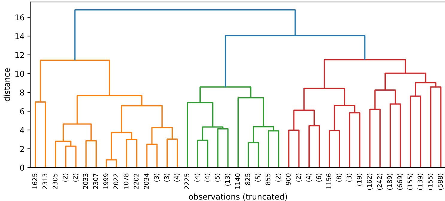
Hierarchical Clustering Dendrogram (Complete Linkage)
