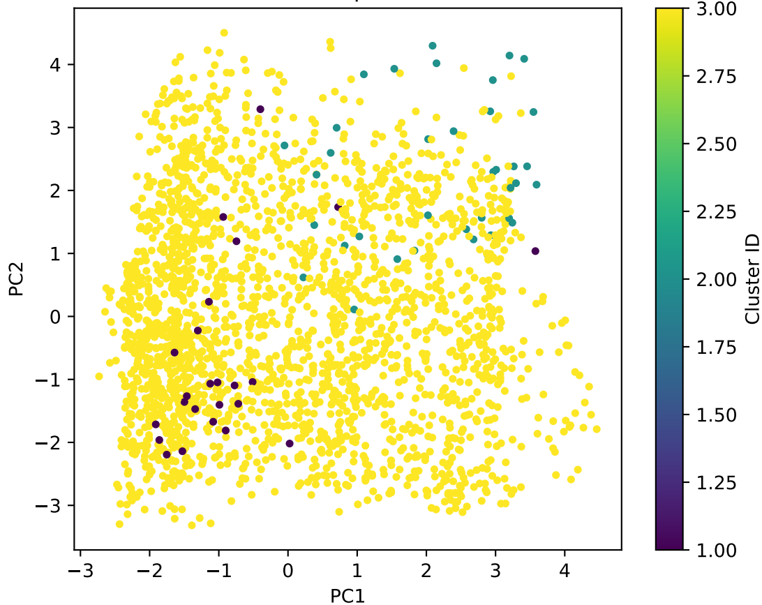
Hierarchical (Complete, 3 clusters)
