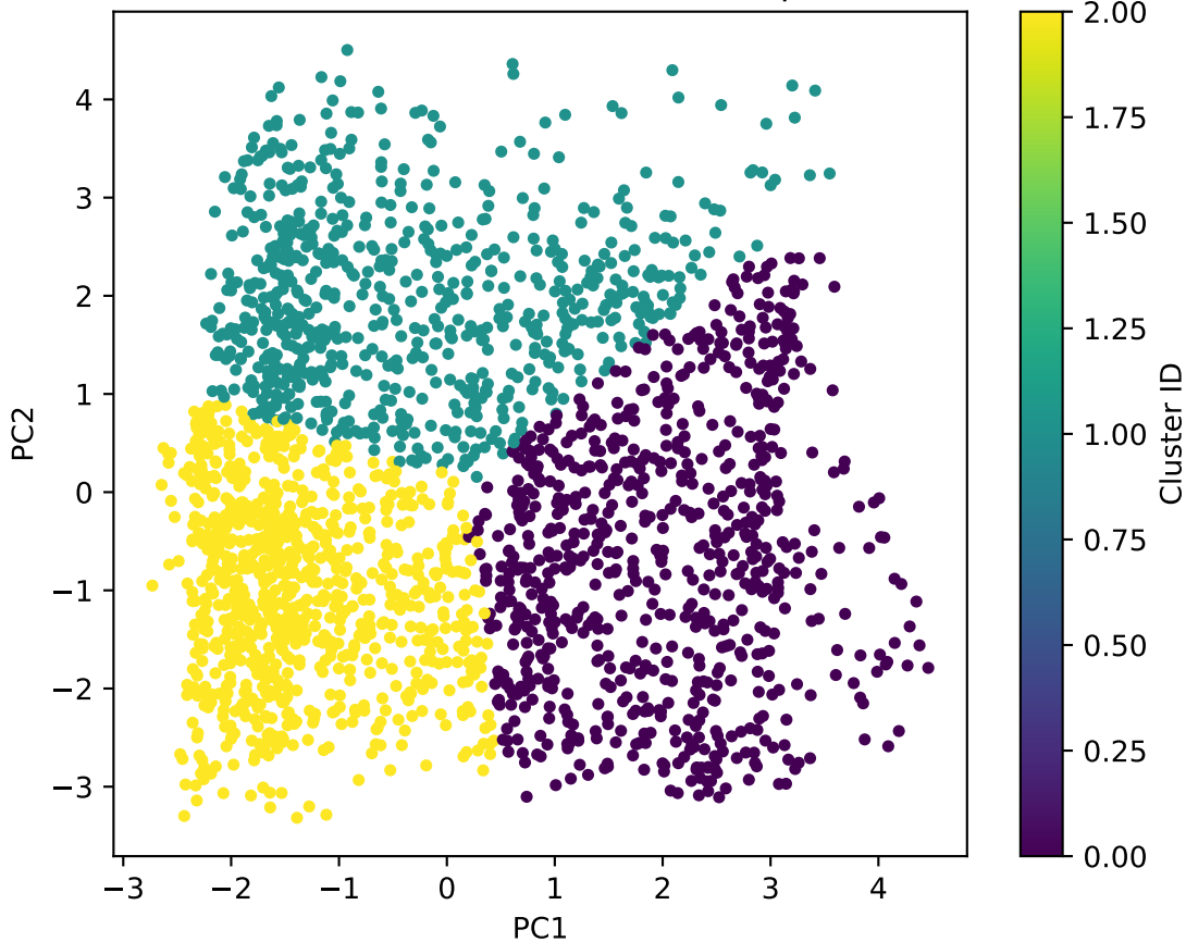
K-Means (k=3) Clusters in PCA Space
