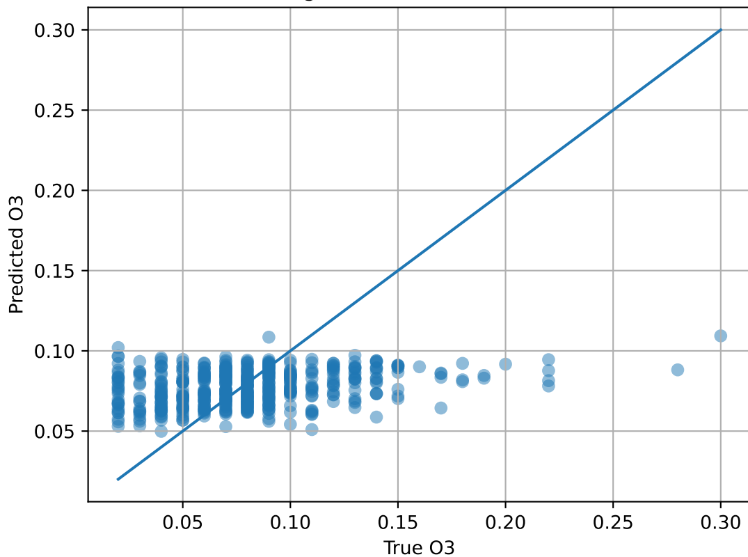
Linear Regression: True vs Predicted O3
