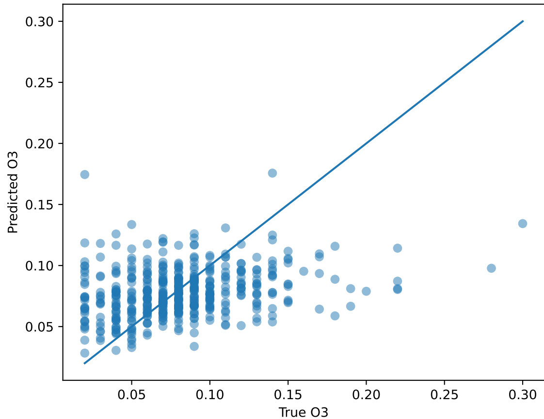
Random Forest
