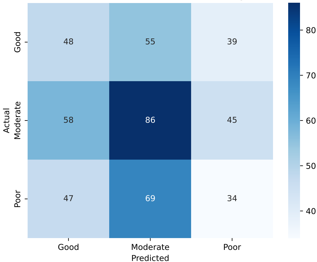
k-NN Confusion Matrix (Second Training)
