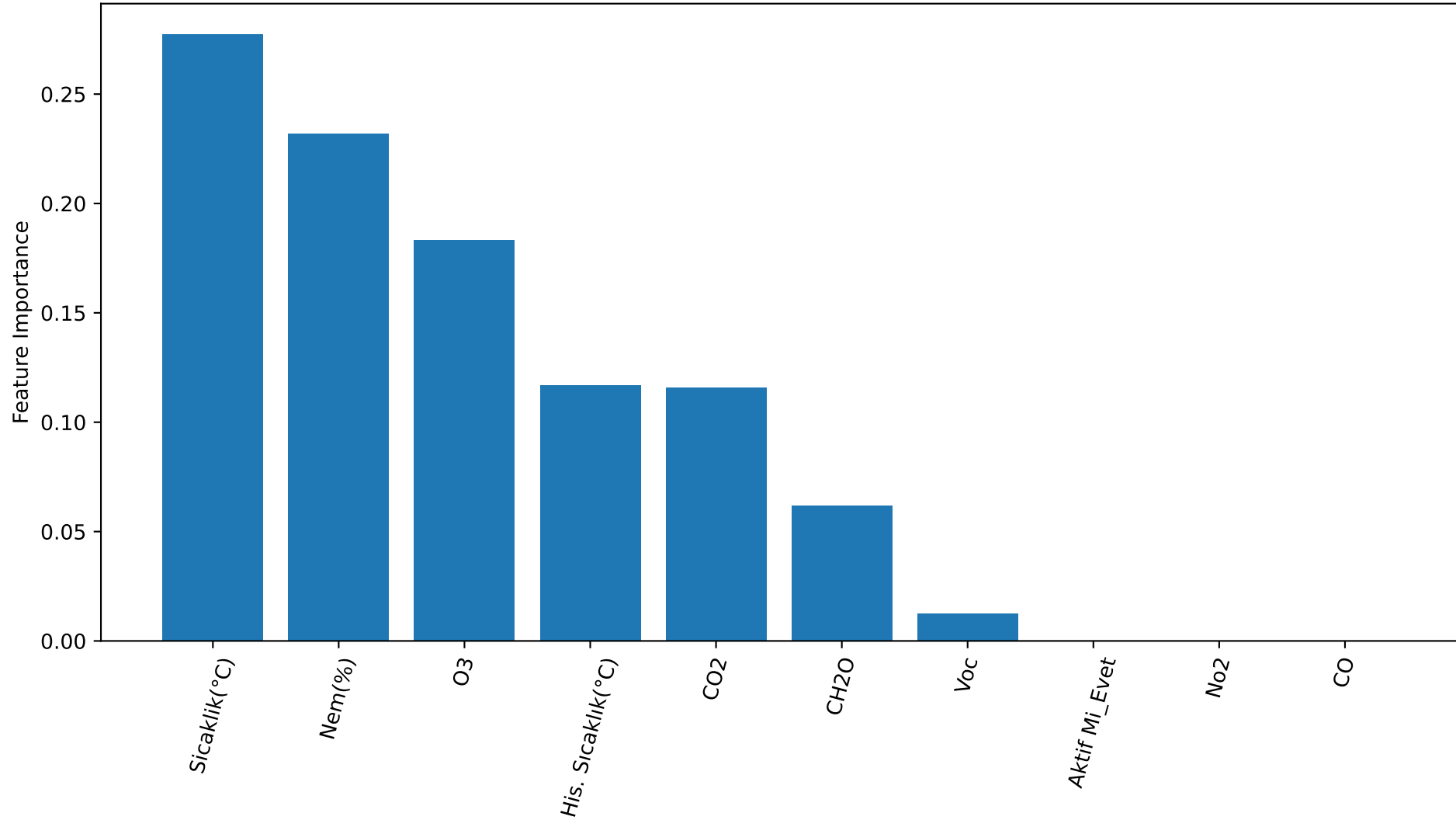
Random Forest Feature Importance (Second Training)
