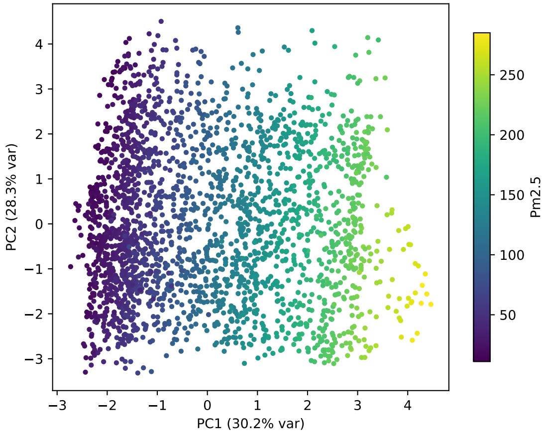
PCA 2D (Standardization)
