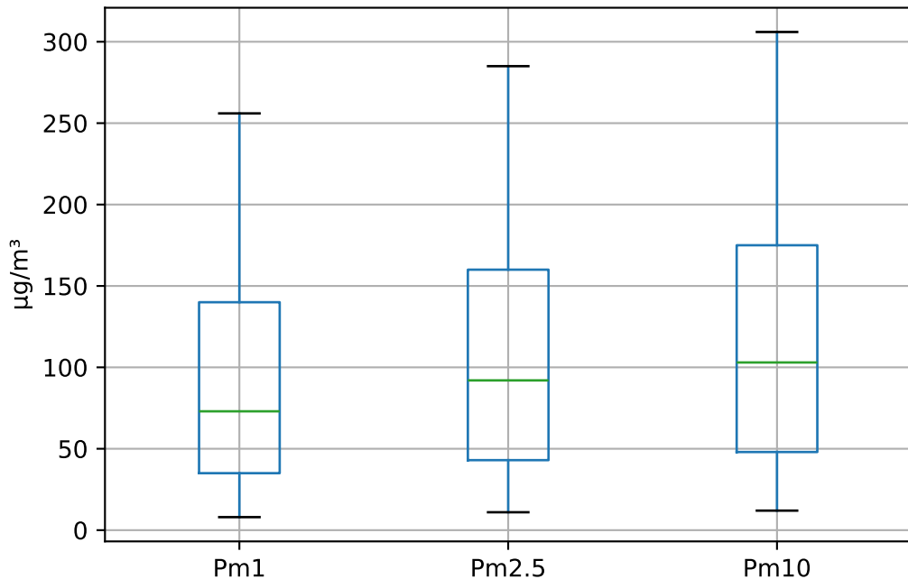
Box Plots of Particulate Matter (PM) Concentrations
