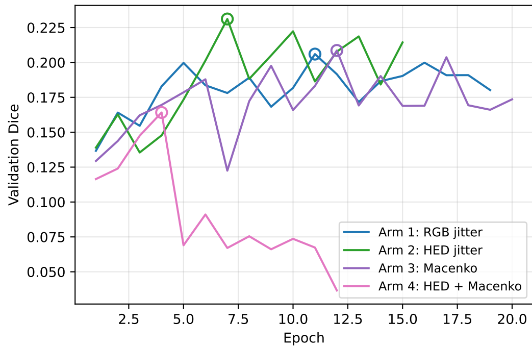
Validation Dice
