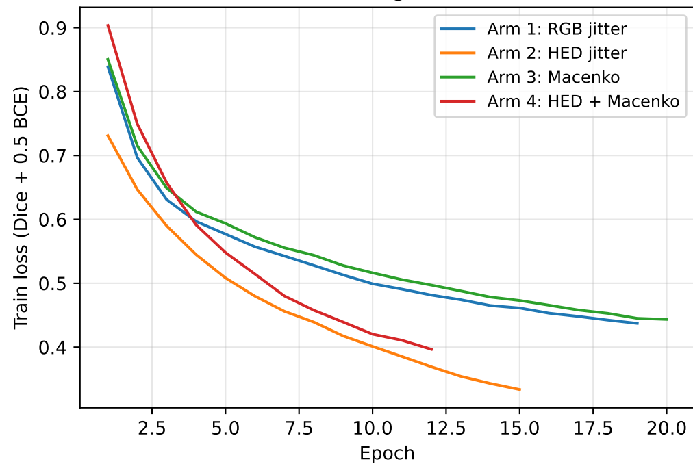
Training loss
