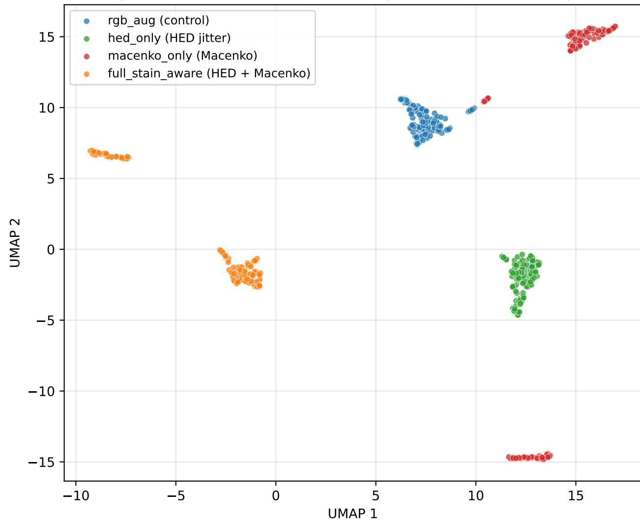
UMAP of layer-4 GAP activations across 4 augmentation arms (val split, seed 42)
