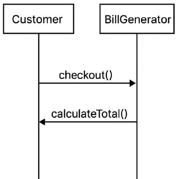
Sequence Diagram
