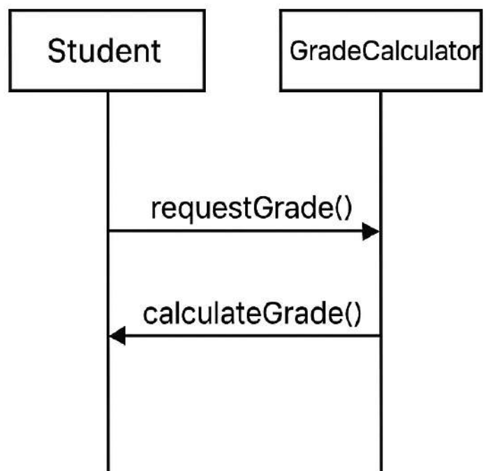
Sequence Diagram
