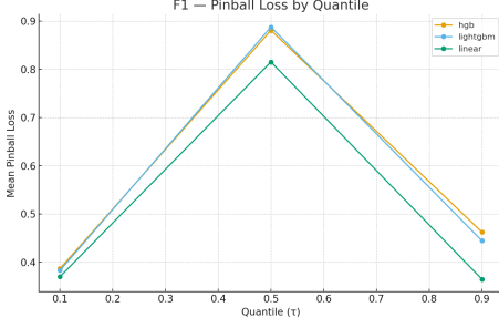
Figure 1: Pinball loss by quantile \tau for baseline models on a synthetic benchmark dataset. Lower values indicate better fit.
