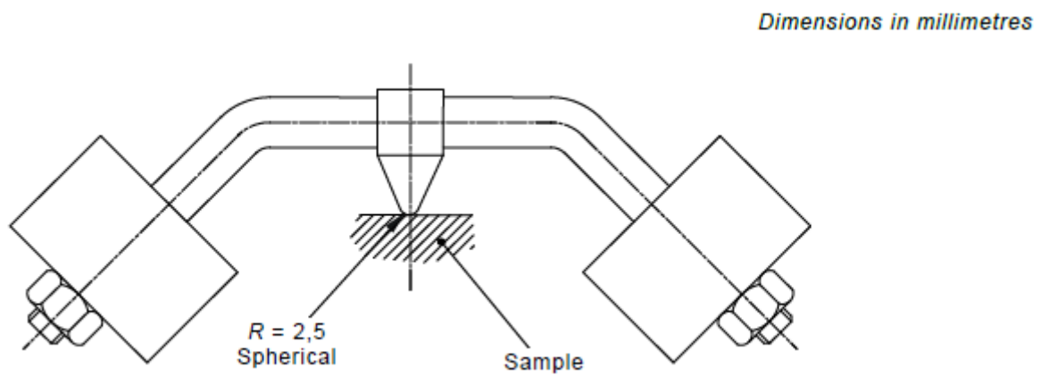
FIG. 23 BALL-PRESSURE APPARATUS
