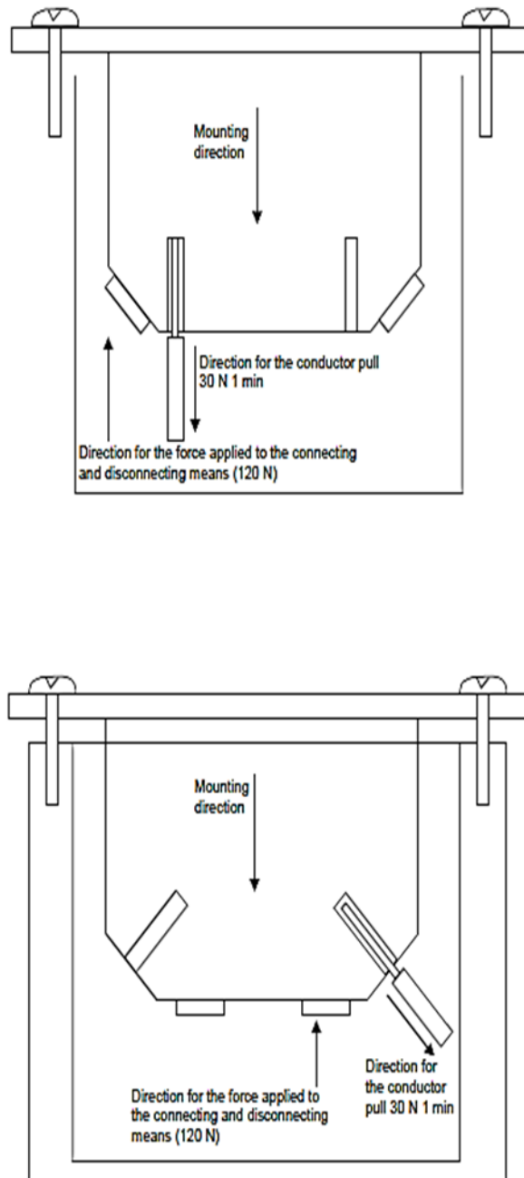
FIG. 13A DETERMINATION OF THE DIRECTION OF THE FORCES TO BE APPLIED
