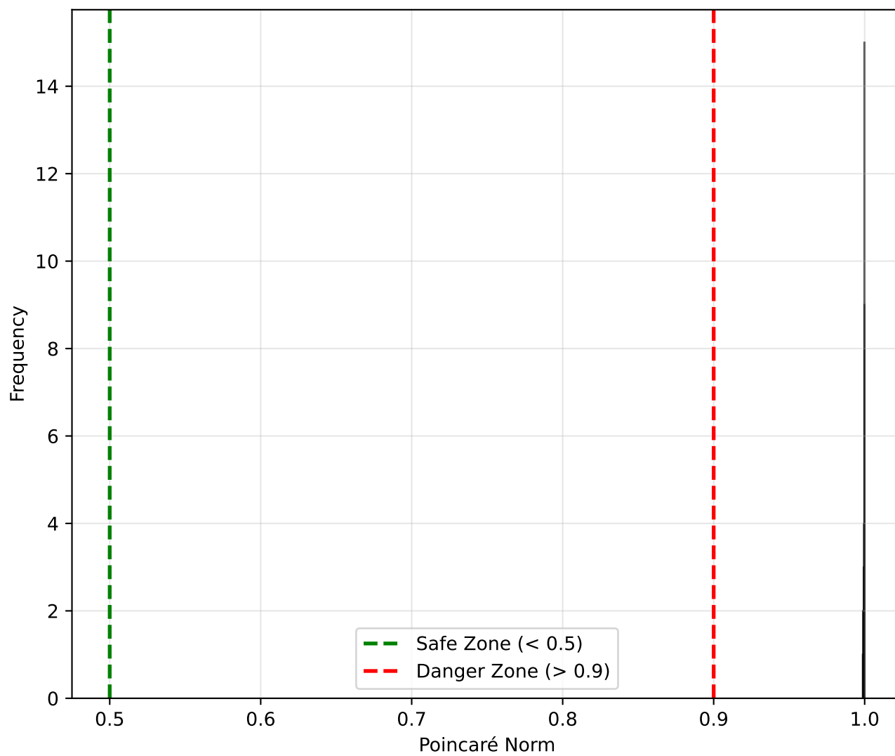
Poincaré Norm Distribution
