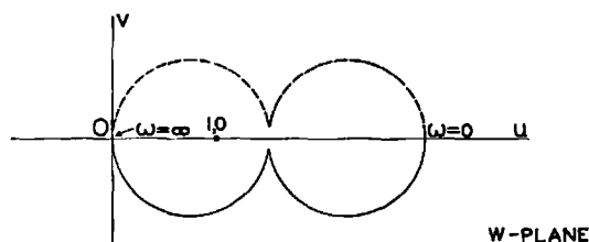
Fig. 9—Illustrating Example 8, with distributed constants.
