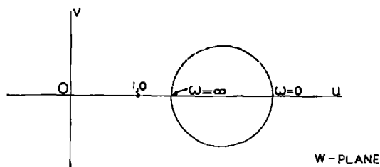
Fig. 8—Illustrating Example 8, without distributed constants.
