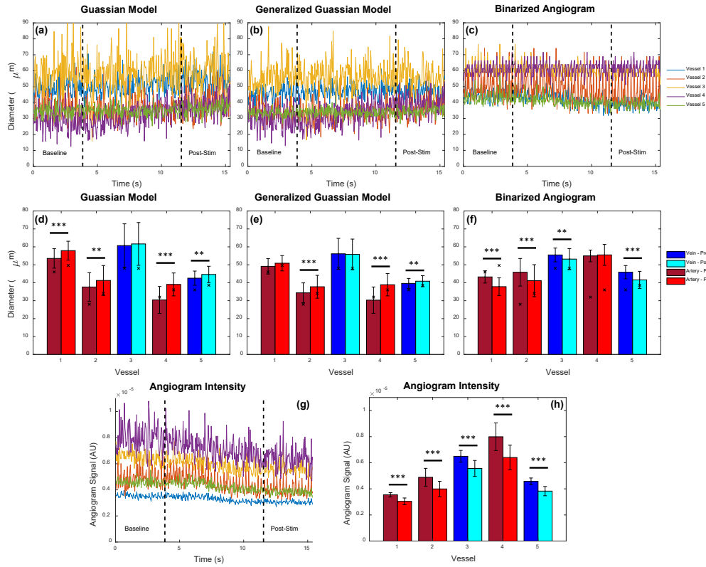
Fig. 8. Functional flicker stimulation results. (a–c) Time series of vessel diameter during baseline and post-stimulation periods for (a) Gaussian model, (b) generalised Gaussian model, and (c) binarised angiogram, across five vessels. Dashed lines indicate stimulation onset and offset. (d–f) Mean diameter per vessel before (dark bars) and after (light bars) stimulation for each method; veins are shown in blue/cyan and arteries in dark/light red. Significance levels: ** p < 0.01 , *** p < 0.001 . (g) Angiogram signal intensity time series and (h) mean intensity per vessel before and after stimulation. Model-based methods detect the expected vasodilation, whereas the binarised method paradoxically reports vasoconstriction.
