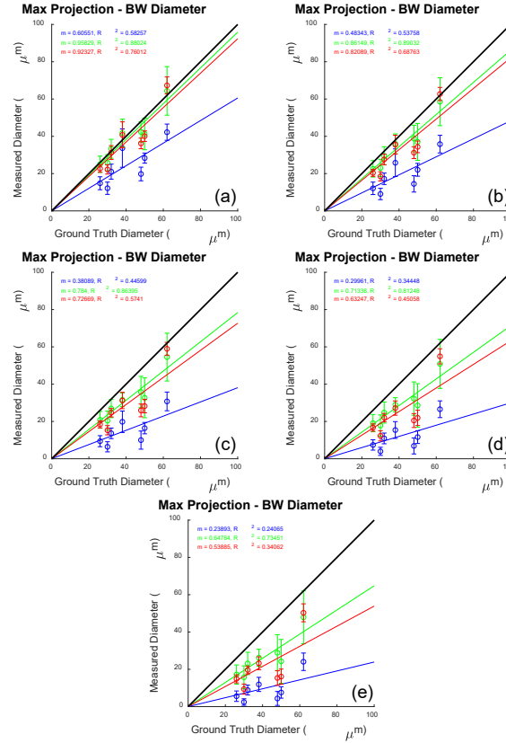
Fig. 5. Vessel diameter measured from BW images versus ground truth for MIP at five threshold levels: (a) BW-1 (lowest) through (e) BW-5 (highest). Regression lines and statistics are shown for pre-contrast (blue), peak contrast (green), and post-contrast (red). Both slope m and R^2 decrease with increasing threshold values.
