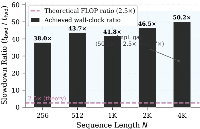
Backward Bottleneck: Achieved vs. Theoretical Slowdown V5 bwd / V4 fwd — Tesla T4, B = 2 , H = 4 , d = 64 , causal
