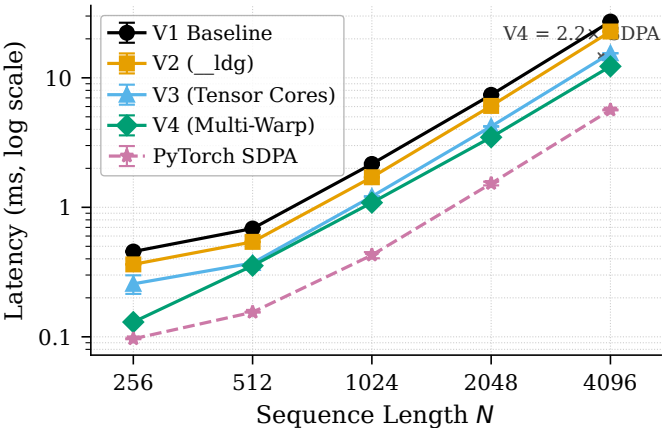
Forward Pass Latency: V1-V4 vs. PyTorch SDPA Tesla T4, B = 2 , H = 4 , d = 64 , causal
