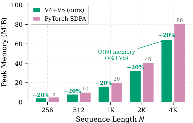
Peak Memory: V4+V5 ( O(N) ) vs. PyTorch SDPA ( O(N^2) ) Tesla T4, B = 2 , H = 4 , d = 64 , causal, backward pass
