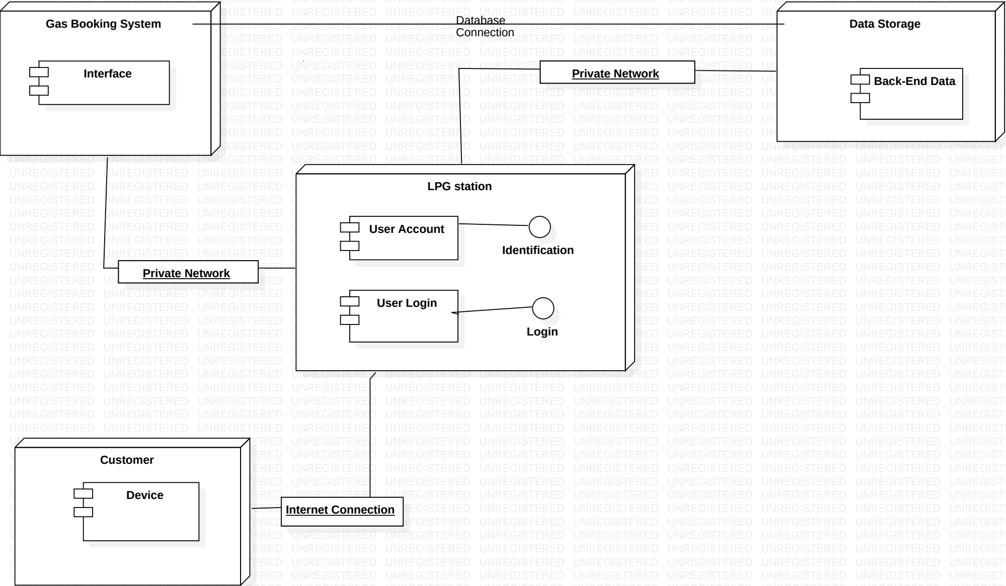
Model1::DeploymentDiagram1
