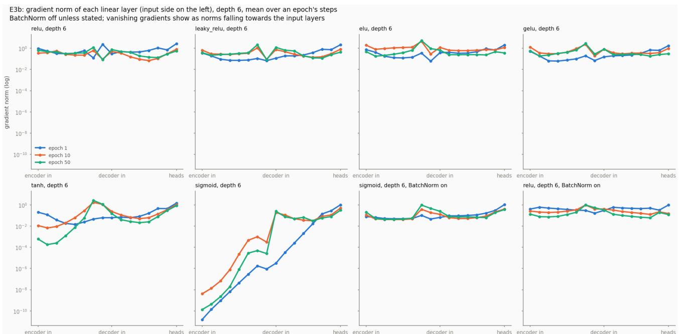
Gradient norms per layer at depth 6
