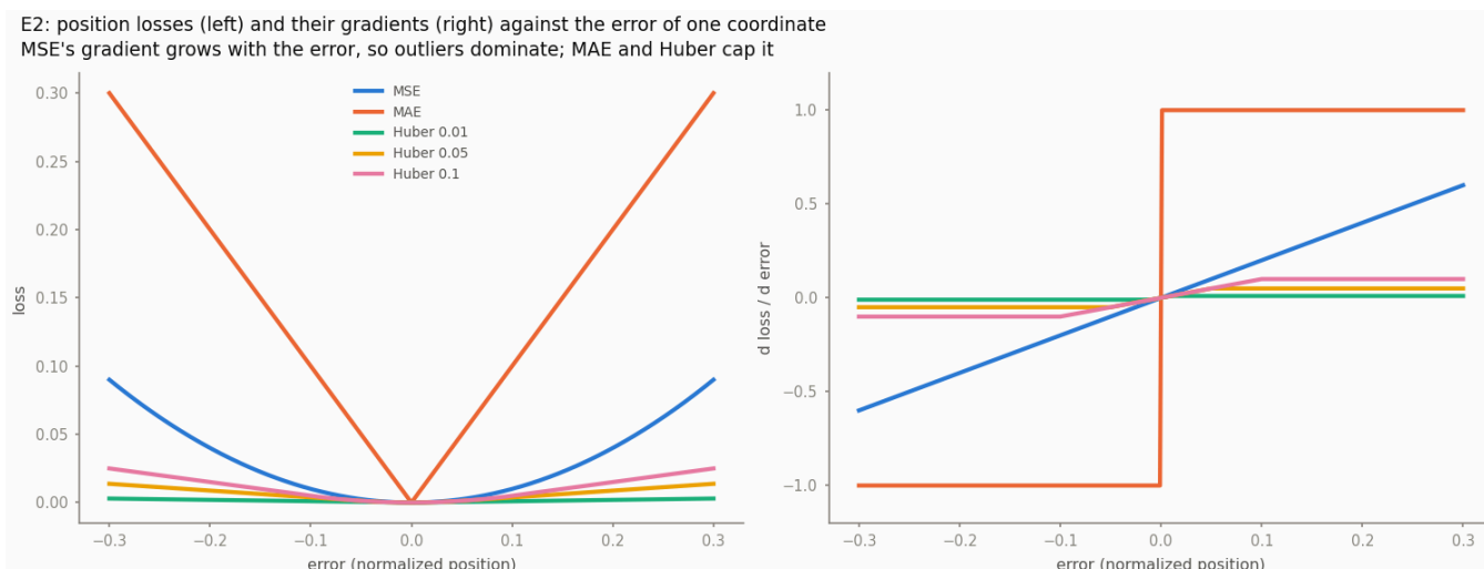
The position losses and their gradients
