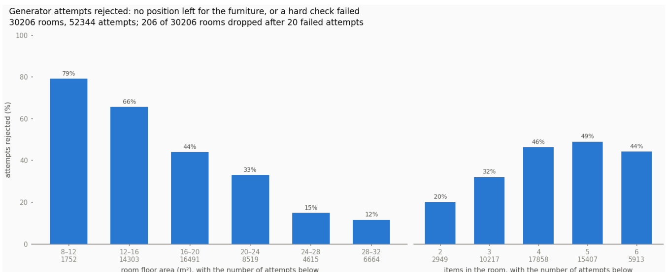
Share of placement attempts rejected, by room area and item count
