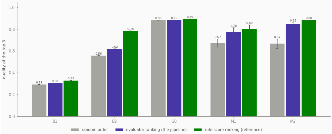
Quality of the top 3 under three rankings
