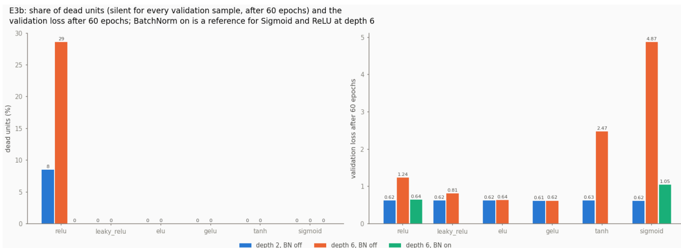
Dead units and loss
