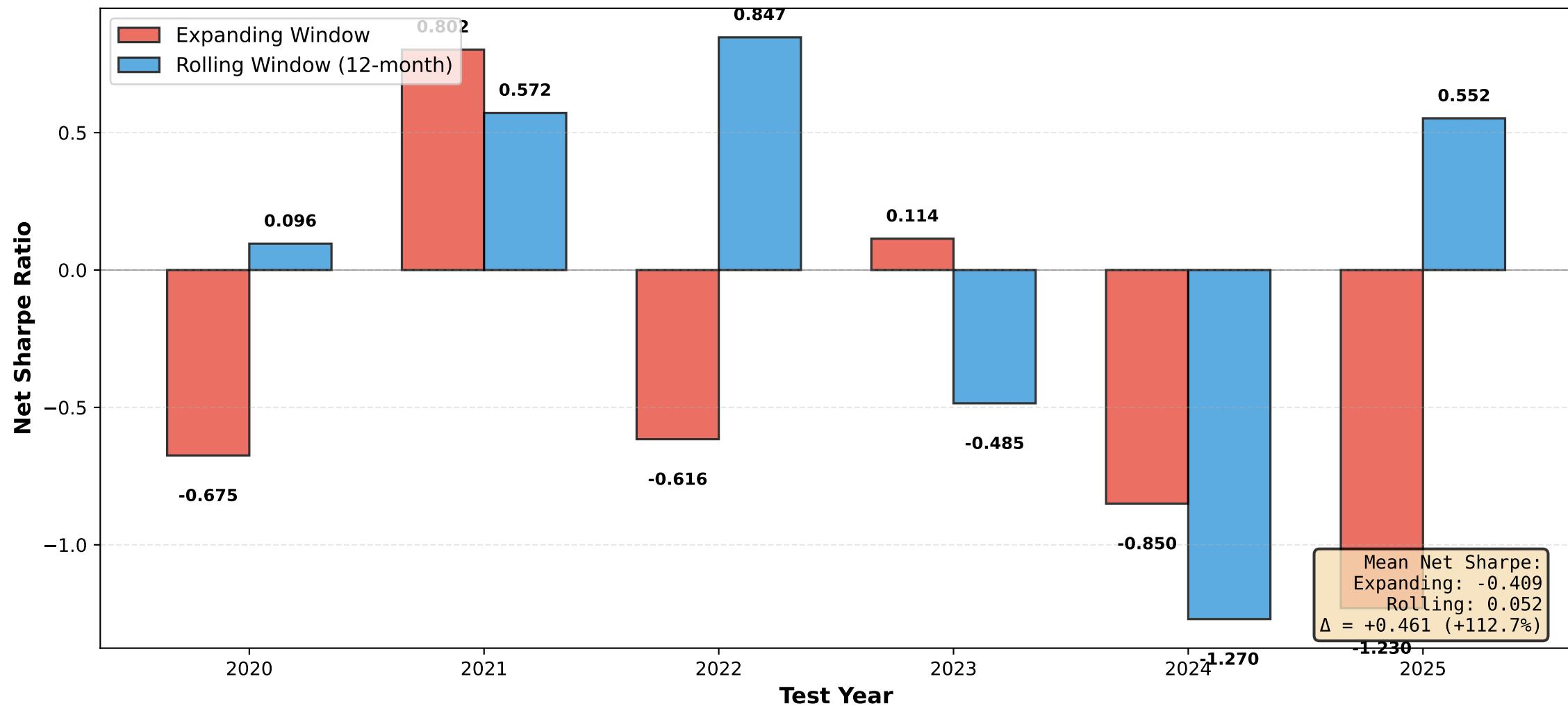
Figure 3.6.1: Walk-Forward Validation — Net Sharpe by Test Year
