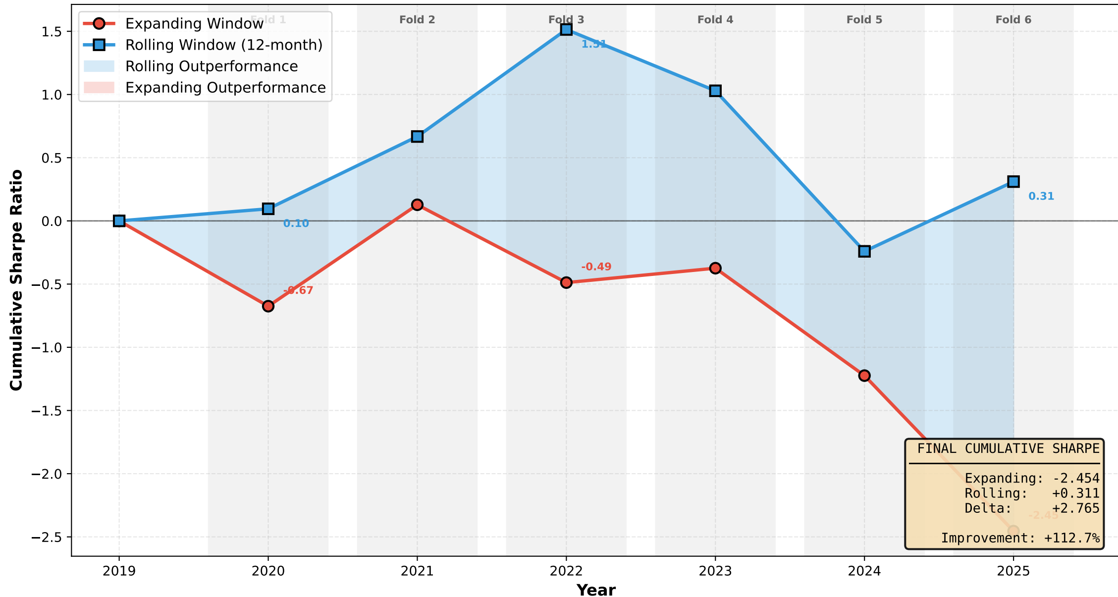
Figure 3.6.4: Cumulative Performance — Expanding vs Rolling Window
