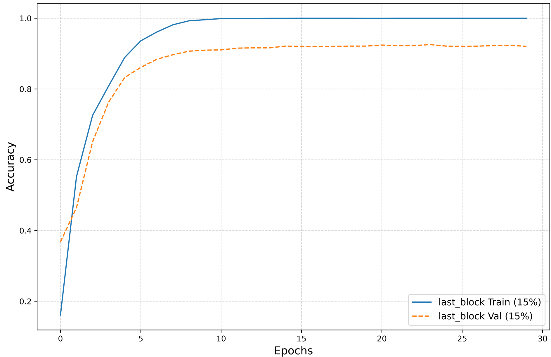
Training and Val Accuracy vs % Unfrozen Parameters - last_block
