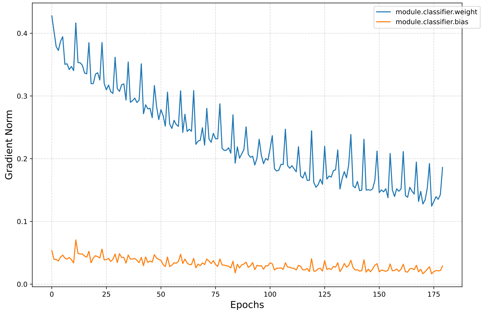
Gradient Norm Statistics Across Layers (linear_probe)
