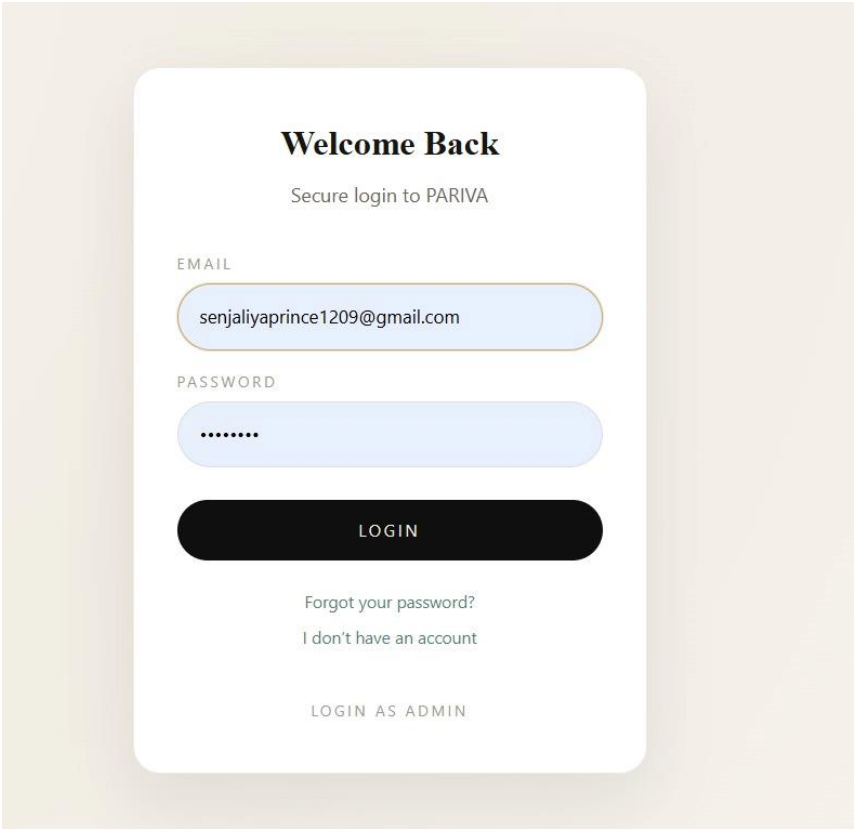
Fig 8.4 User Login
