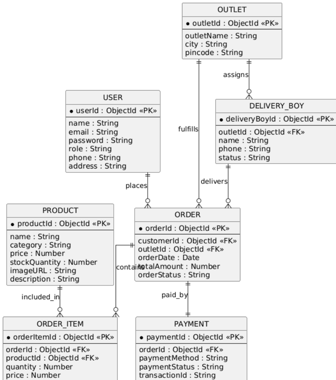
Fig 5.4 Database Relationship Diagram
