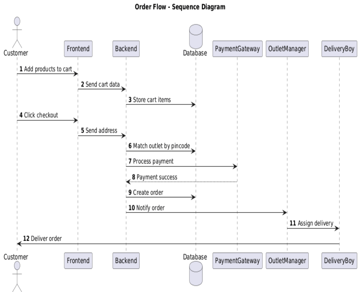
Fig 4.4 Sequence Diagram
