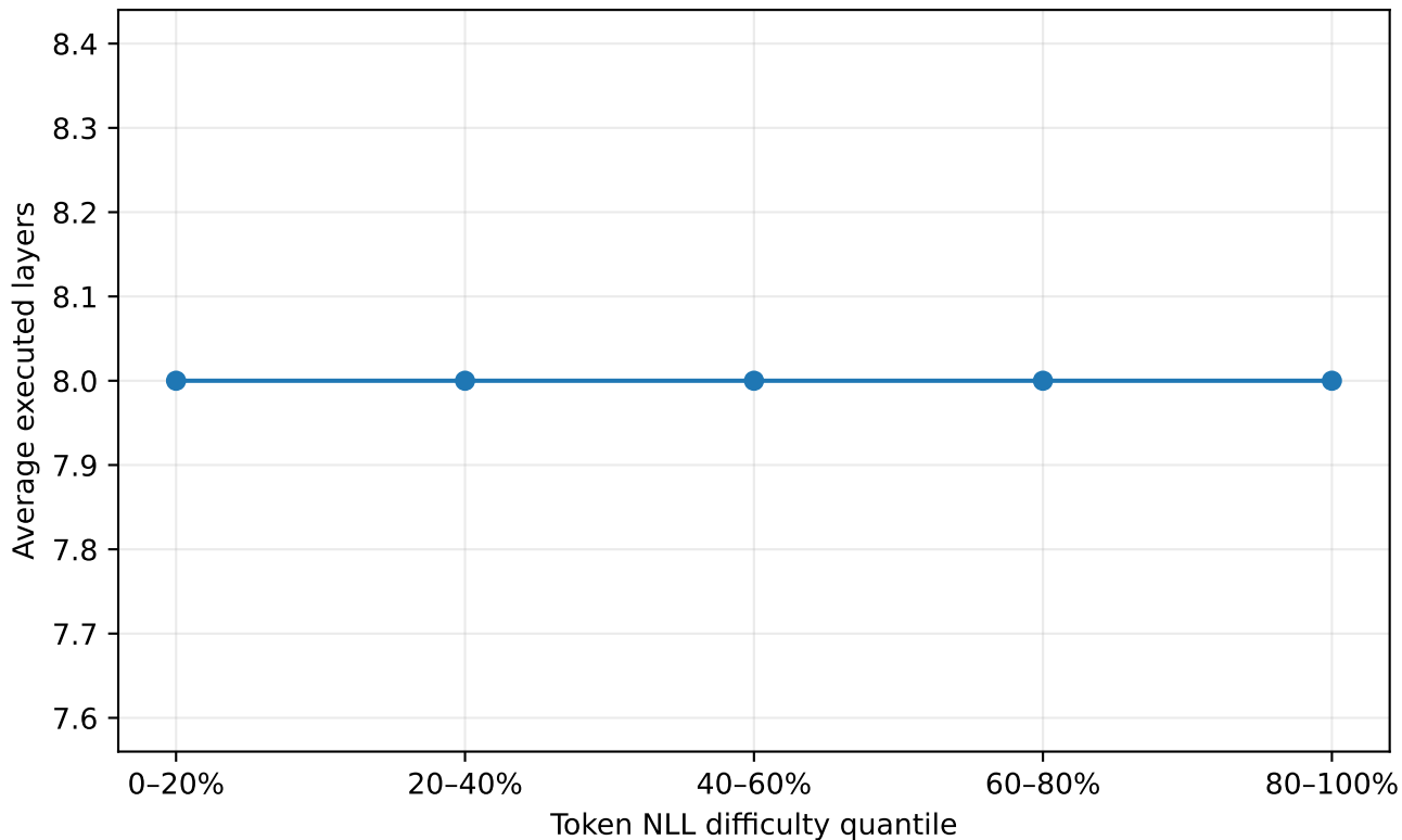
Token difficulty versus dynamic depth
