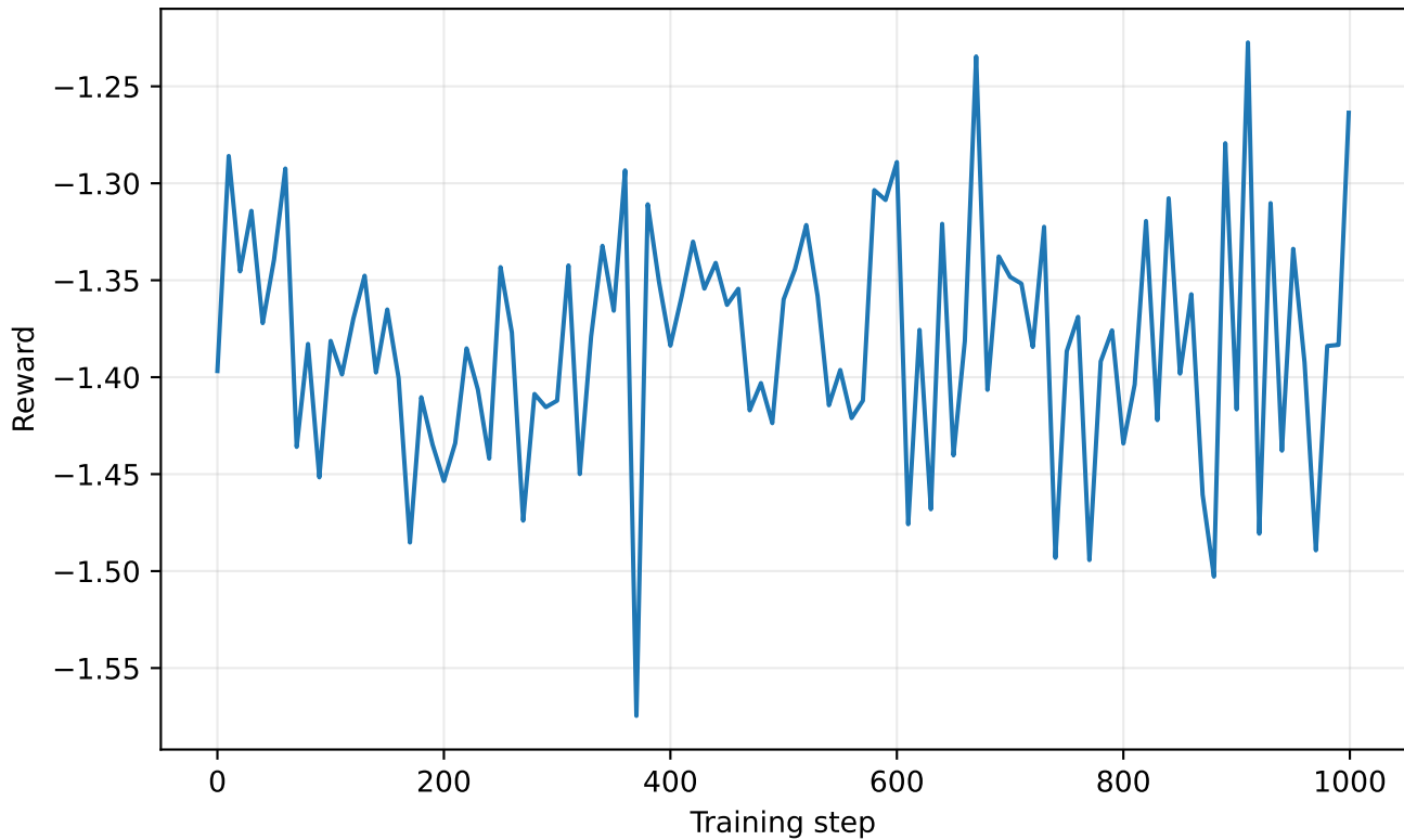
GRPO reward
