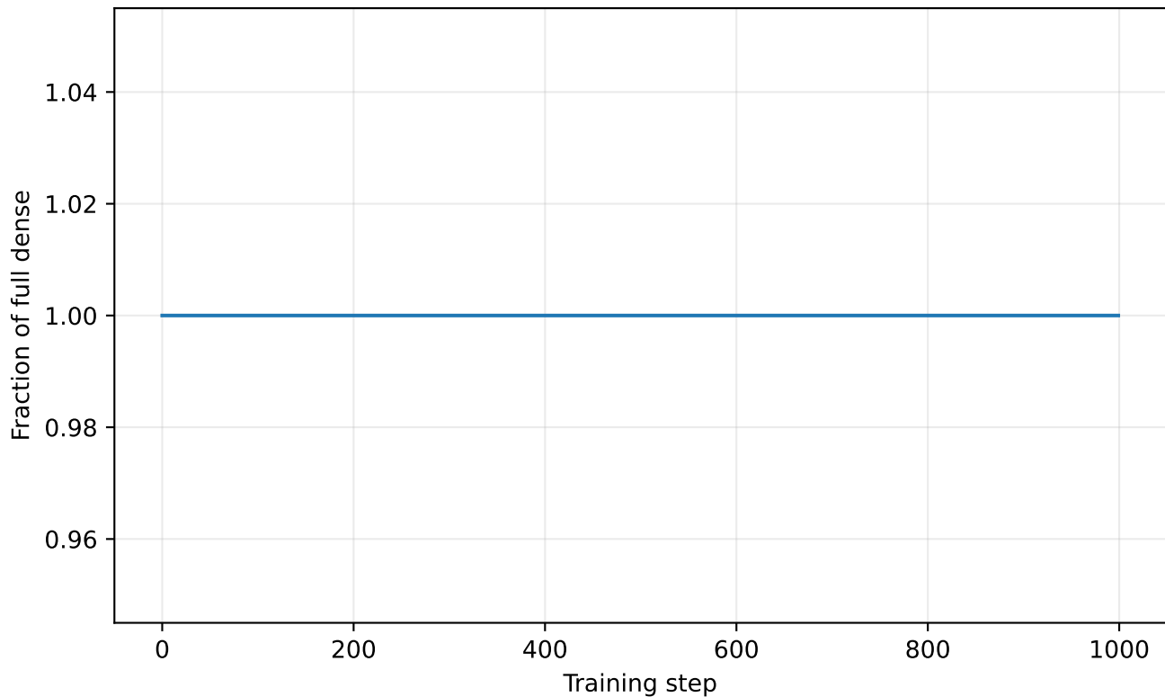
Estimated FLOPs
