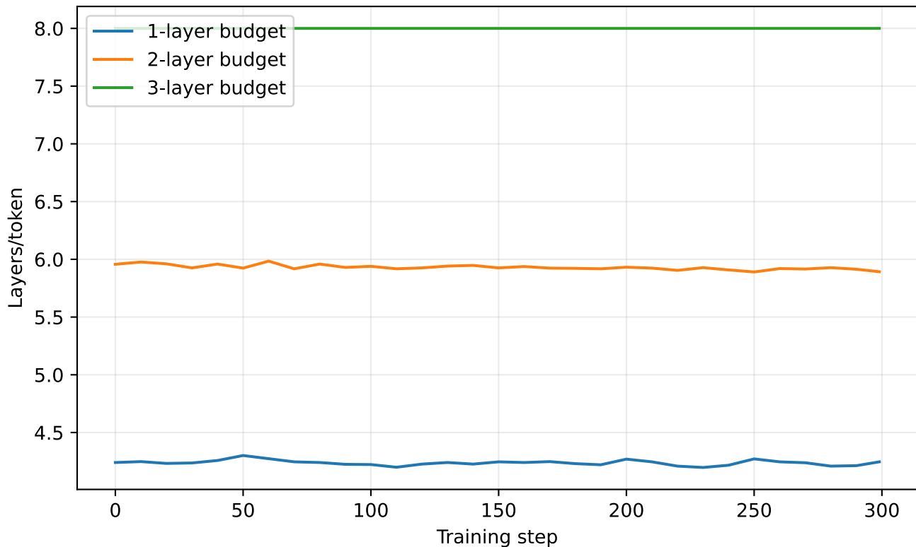
Achieved rollout depths
