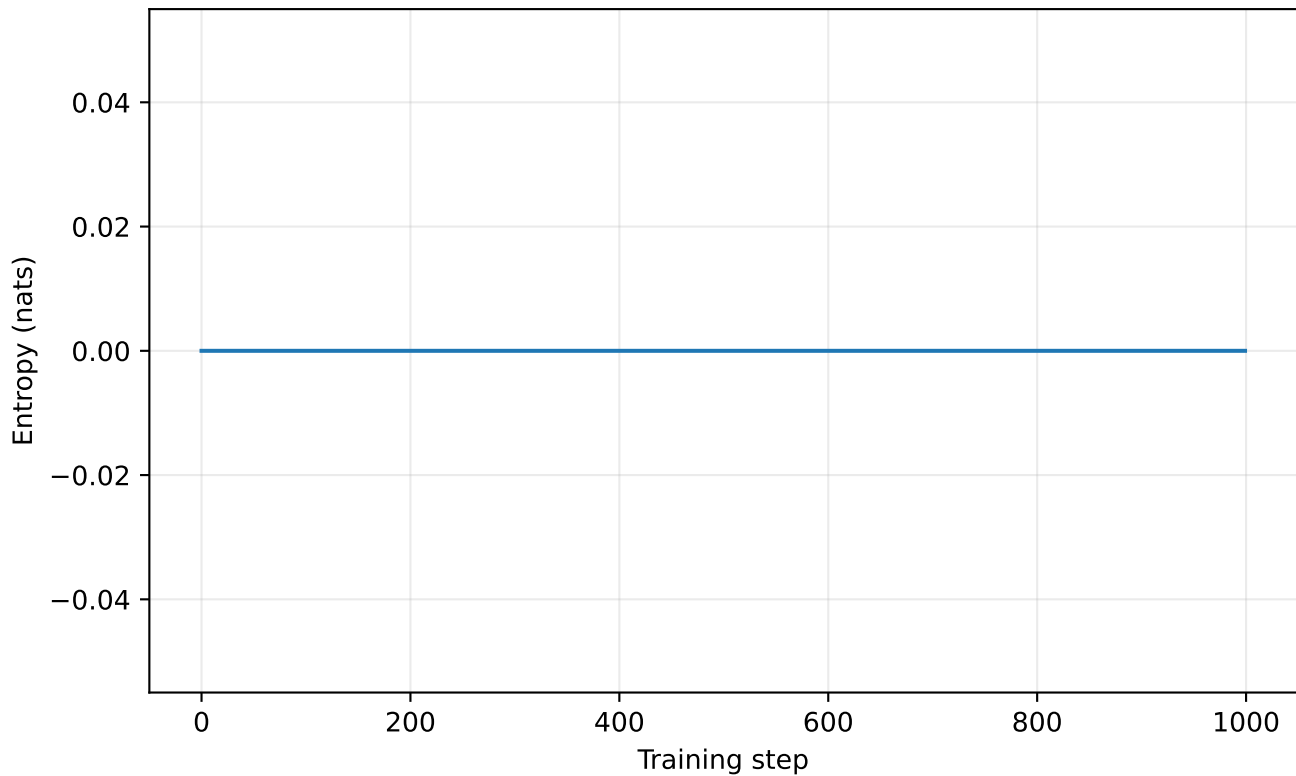
Routing entropy
