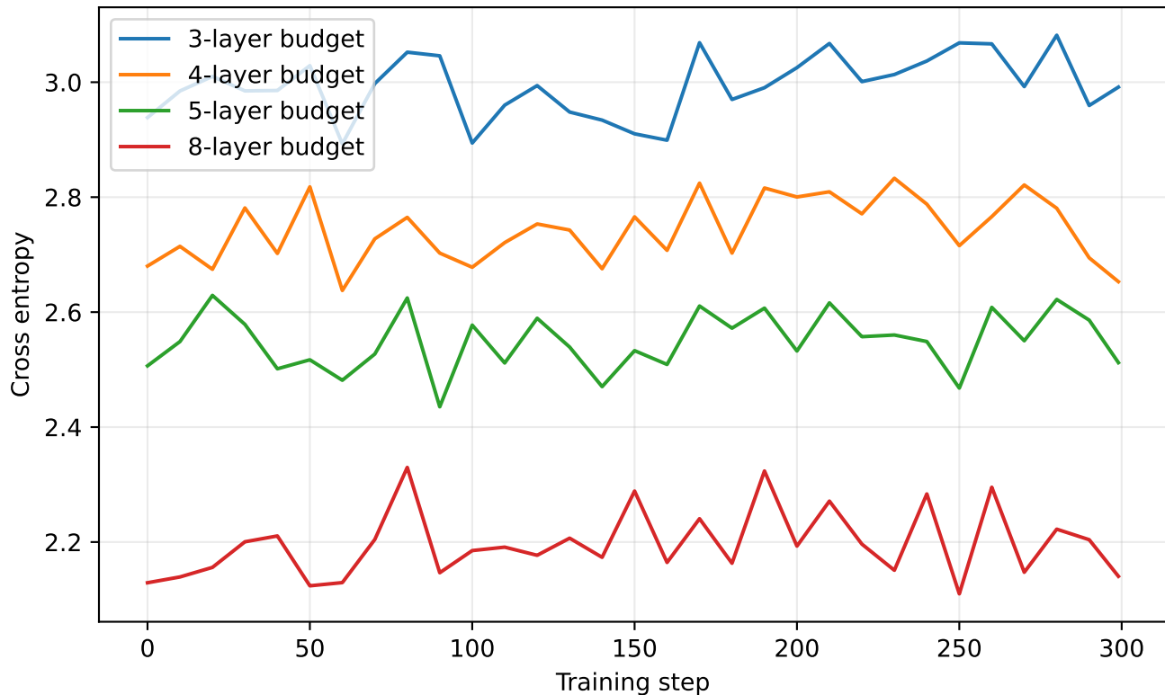
Cross entropy by rollout budget
