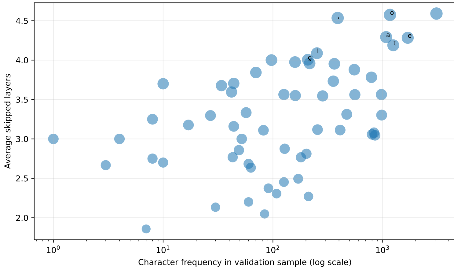
Token-wise SkipLayer behavior
