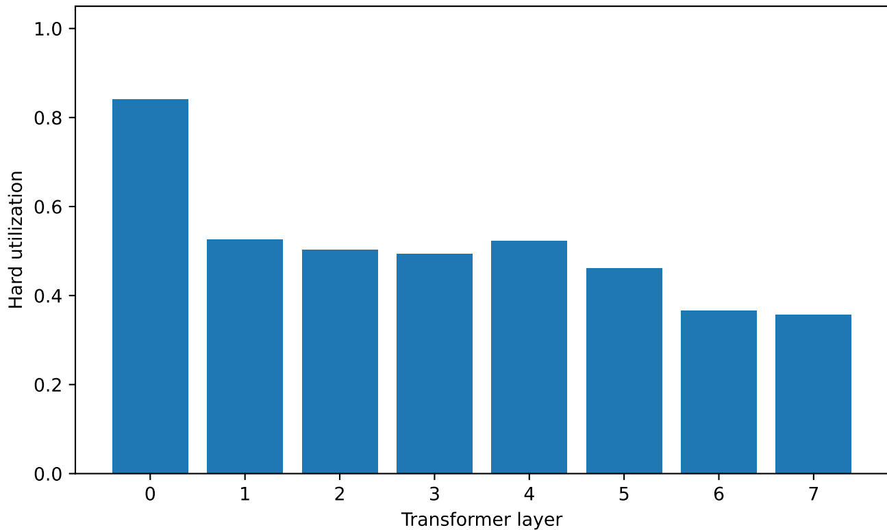
Per-layer utilization
