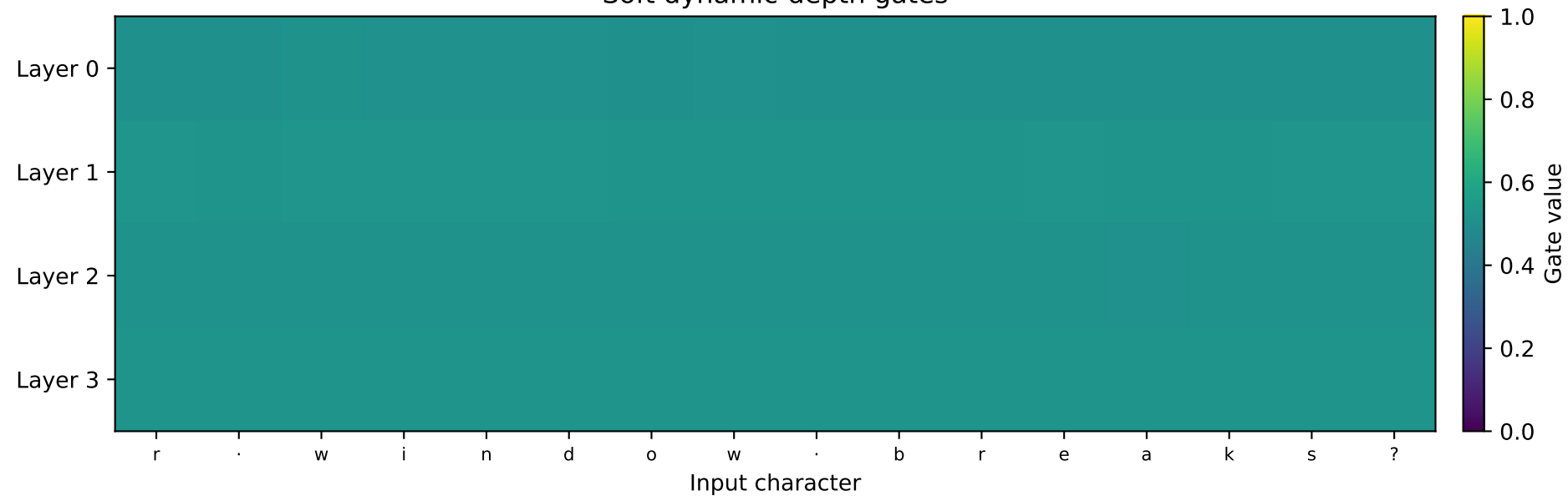
Soft dynamic-depth gates
