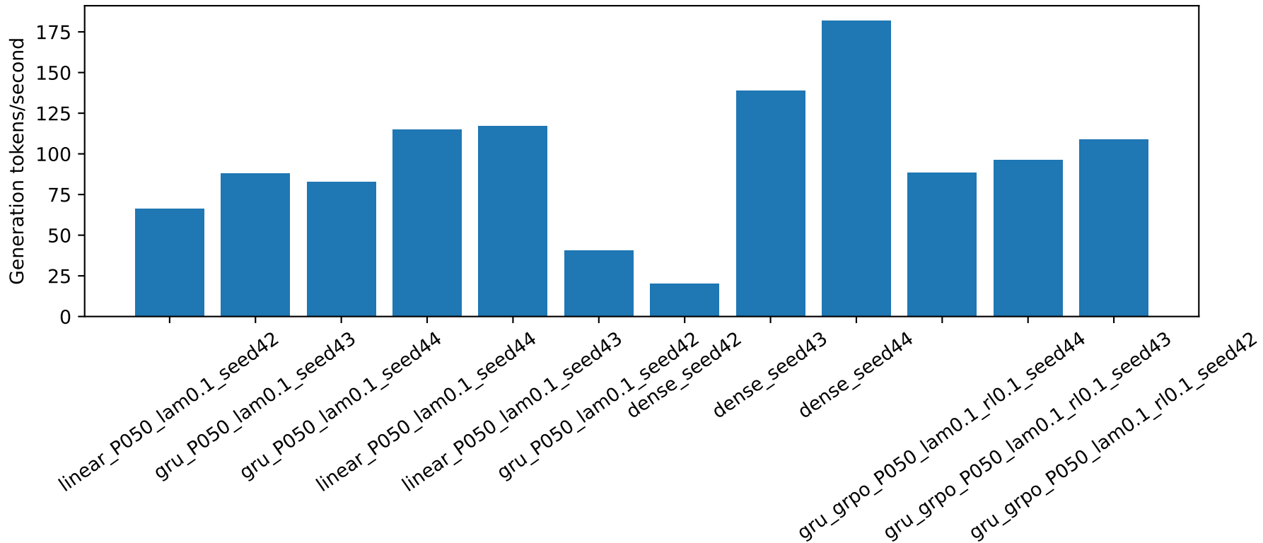
Generation tokens/second
